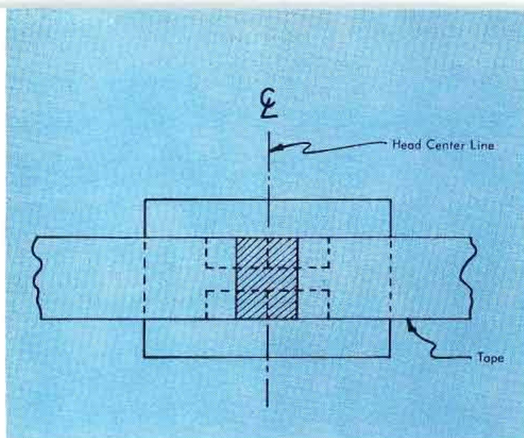
Figure 5. Proper Tape Contact Area (Front View)
