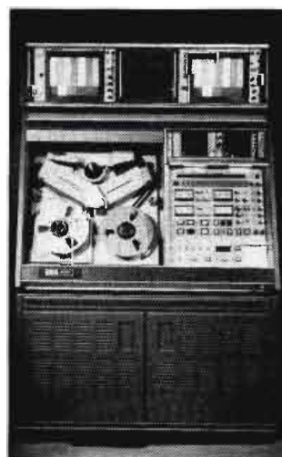
IVC-9000 BROADCAST VIDEO-TAPE RECORDER —New, two-inch, segmented scan VTR, the most significant development in VTR's since broadcast recorders were first introduced. Picture quality better than 15 ips quad. Economy better than 7½ ips quad.
